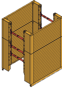
KRINGS KS 100 Manhole Rec. shoring depth: max. 4.00 m Page 16
