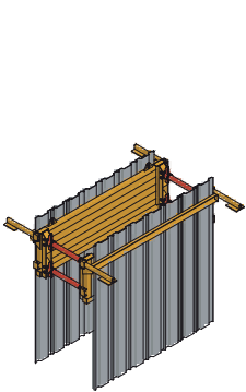
KRINGSBLU Rec. shoring depth: max. 2.50 m Page 28
