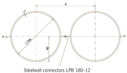
Steelwall connectors LPB 180-12
